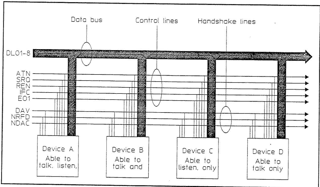
Figure 2-1. HP-IB Structure
